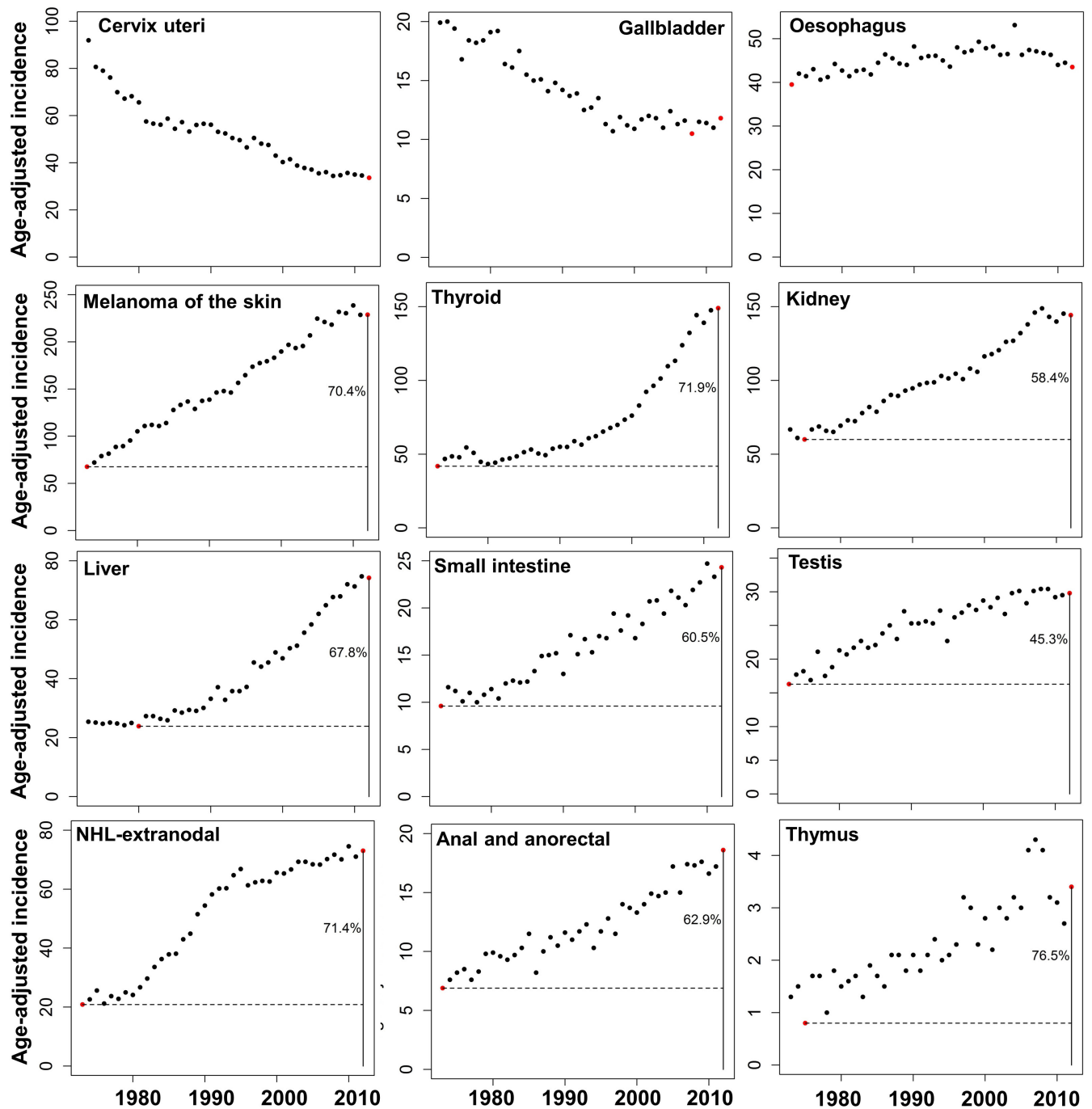
Extended Data Figure 1 | Examples of increased cancer incidence trends from 1973–2012 in SEER data. The cancer types include melanoma, thyroid cancer, kidney cancer, liver cancer, small intestine cancer, testicular cancer, non-Hodgkin lymphoma (NHL), anal and anorectal cancer and thymus cancer. The horizontal dashed lines indicate the
