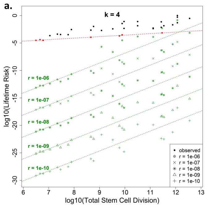
Extended Data Figure 3 | Sensitivity analysis of different mutation rates on tLIR when the number of hits ( k ) required is 4. a, b, Theoretical intrinsic lifetime risks (tLIR) for cancers have been calculated based on five different mutation rates: r = 1 \times 10^{-10} , 1 \times 10^{-9} , 1 \times 10^{-8} , 1 \times 10^{-7} , 1 \times 10^{-6} . The red dashed lines are the ‘intrinsic’ risk lines based on the
