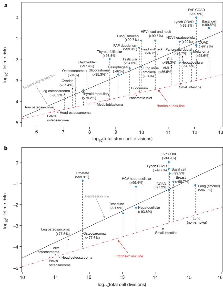
Figure 3 | Estimation of the proportion of lifetime cancer risk that is not due entirely to ‘bad luck’. a , Estimations based on total tissue stem-cell divisions originally reported in Tomasetti & Vogelstein 5 and total tissue cell divisions ( b ). Red dots are cancers used to compute the ‘intrinsic’ risk
