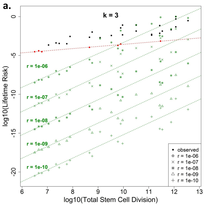
Extended Data Figure 2 | Sensitivity analysis of different mutation rates on tLIR when the number of hits ( k ) required is 3. a, b, Theoretical intrinsic lifetime risks (tLIR) for cancers have been calculated based on five different mutation rates: r = 1 \times 10^{-10} , 1 \times 10^{-9} , 1 \times 10^{-8} , 1 \times 10^{-7} , 1 \times 10^{-6} . The red dashed lines are the ‘intrinsic’ risk lines based on the
