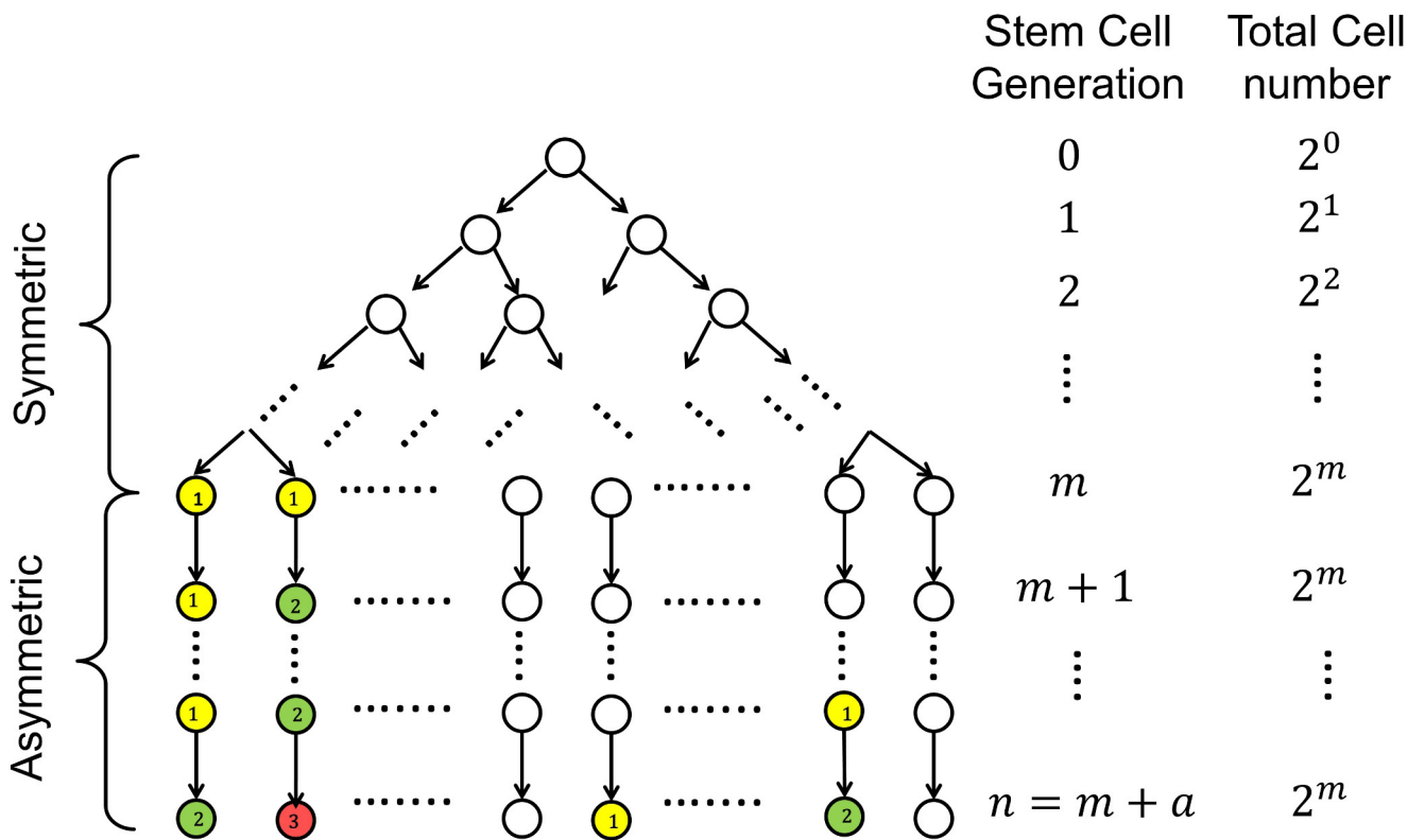
Extended Data Figure 5 | Intrinsic cancer risk modelling. Part 2 of 2: schema of stem-cell divisions and driver gene mutations, from which the theoretical lifetime intrinsic risks (tLIR) for cancer due to k driver gene mutations are computed. Each coloured circle represents the mutation of a new driver gene in the given stem cell (yellow, first mutation; green,
